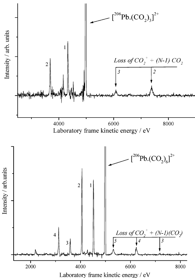
Figure 2. Fragmentation patterns of [^{206}\text{Pb}(\text{CO}_2)_N]^{2+} complexes for N = 3 and 6 following collisional activation. The values shown correspond to the numbers of neutral ligands lost as a consequence of collisional activation, with features associated with charge-transfer processes being shown in italics. For certain values of N there is a mass coincidence with an underlying singly charged ion, which, in the case of N = 6 , is responsible for the unexpected alternation in neutral ligand loss from the doubly charged ion.
